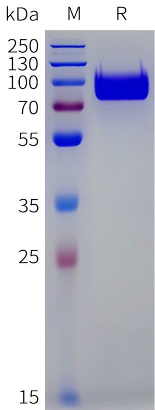
Figure 1. Human SIRPα V8 Protein, hFc Tag on SDS-PAGE under reducing condition.
