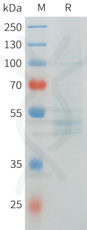
Figure 1. Human RNF133 Protein, hFc Tag on SDS-PAGE under reducing condition.
