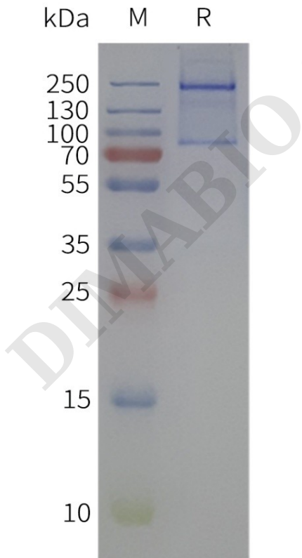
Figure 2. Human PTPRZ1-Nanodisc, Flag Tag on SDS-PAGE
