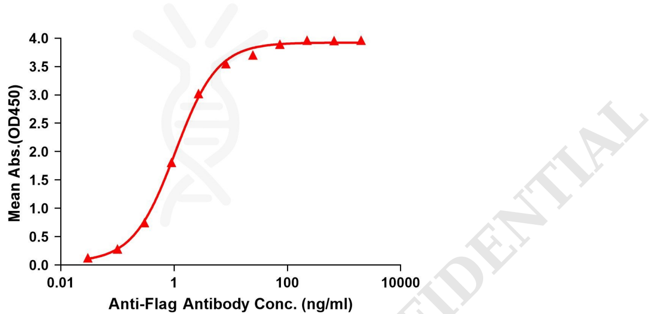
Figure 1. Elisa plates were pre-coated with Flag Tag PTPRZ1-Nanodisc (0.2µg/per well). Serial diluted anti-Flag monoclonal antibody solutions were added, washed, and incubated with secondary antibody before Elisa reading. From above data, the EC50 for anti-Flag monoclonal antibody binding with PTPRZ1-Nanodisc is 1.047ng/ml.
