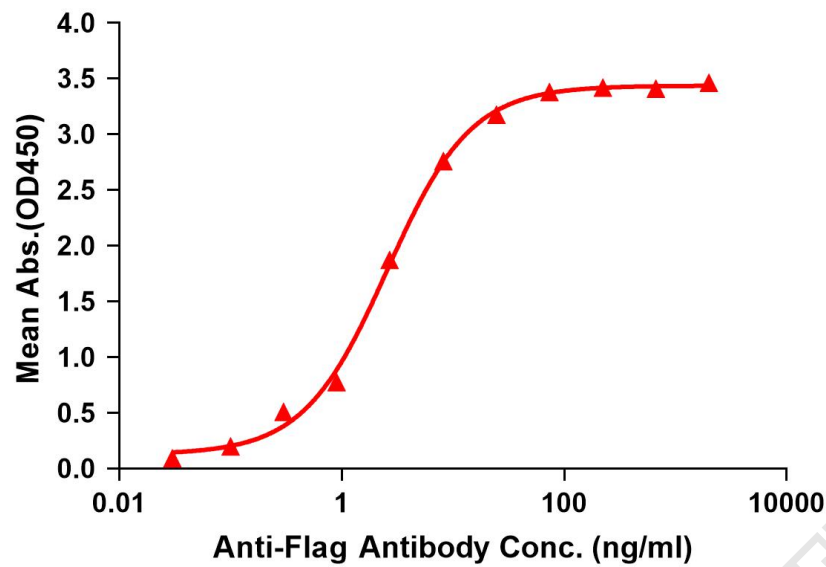
Figure 1. Elisa plates were pre-coated with C-Flag&Strep Tag NK2R-Strep-Nanodisc (0.2µg/per well). Serial diluted anti-Flag monoclonal antibody solutions were added, washed, and incubated with secondary antibody before Elisa reading. From above data, the EC50 for anti-Flag monoclonal antibody binding with NK2R-Strep-nanodisc is 2.571ng/ml.
