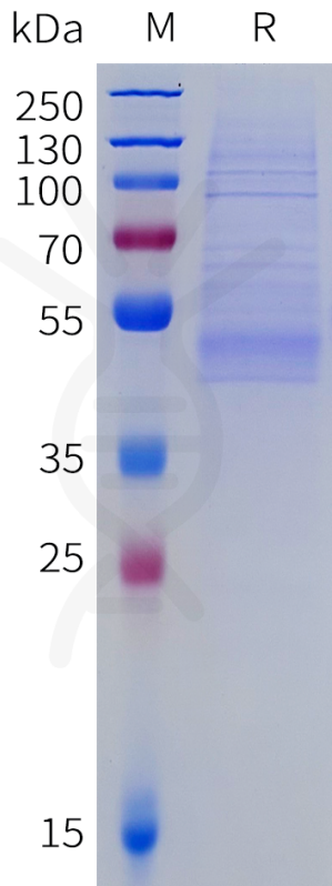
Figure 1. Cynomolgus IL11RA Protein, His Tag on SDS-PAGE under reducing condition.
