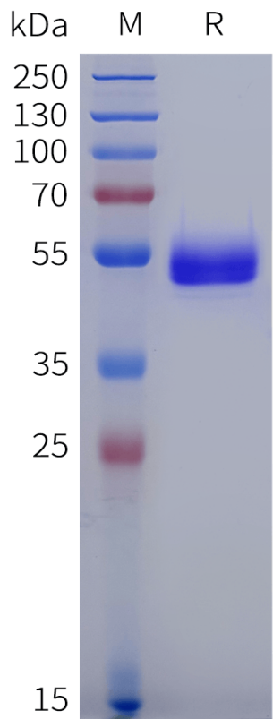
Figure 1. Canine IL31 Protein, hFc Tag on SDS-PAGE under reducing condition.
