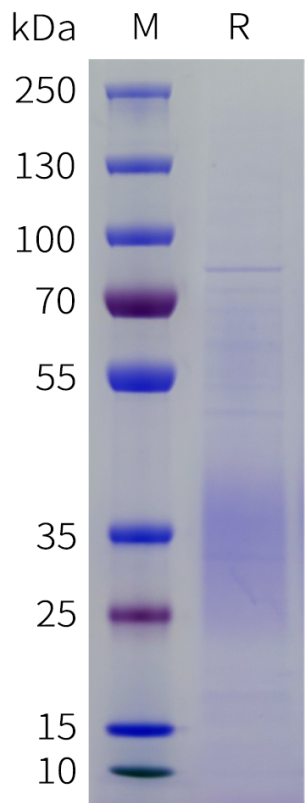
Figure 1. Biotinylated Human ACVR2B(19-137) Protein, His Tag on SDS-PAGE under reducing condition.
